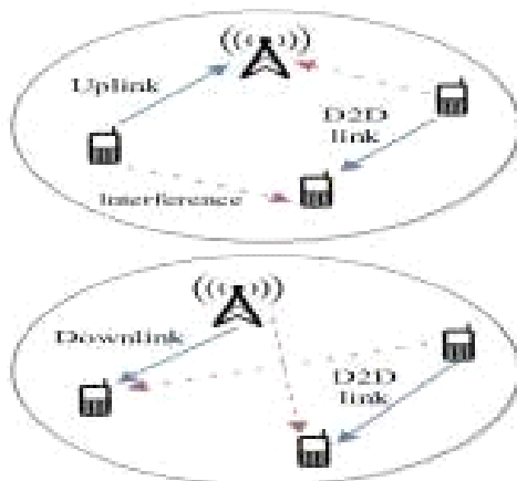
Fig: 5. D2D using cellular uplink and downlink resources
