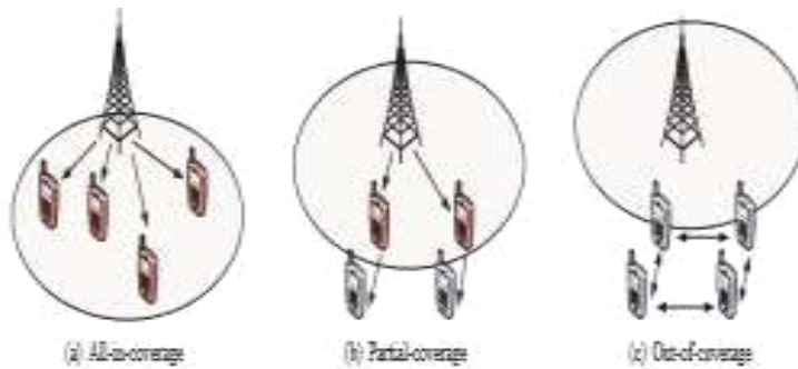
Fig: 2. Three synchronization scenarios in D2D network
